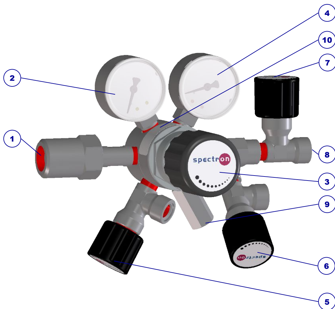
Illustration 1: Pressure regulator design FE51-SP
