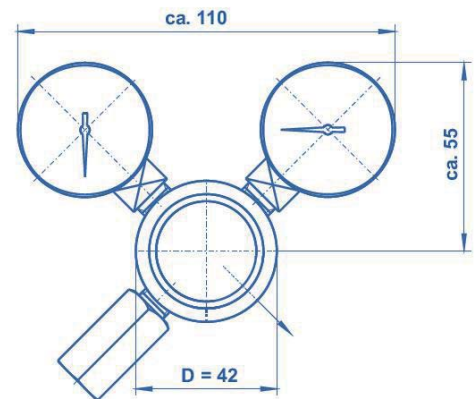
Main dimensions
