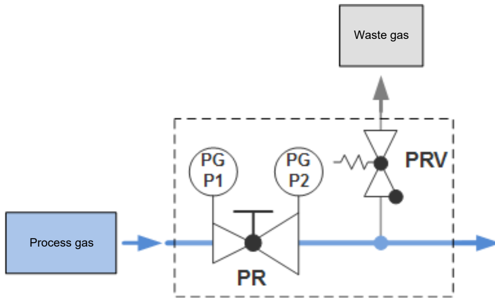
Illustration 2: P&ID M52
