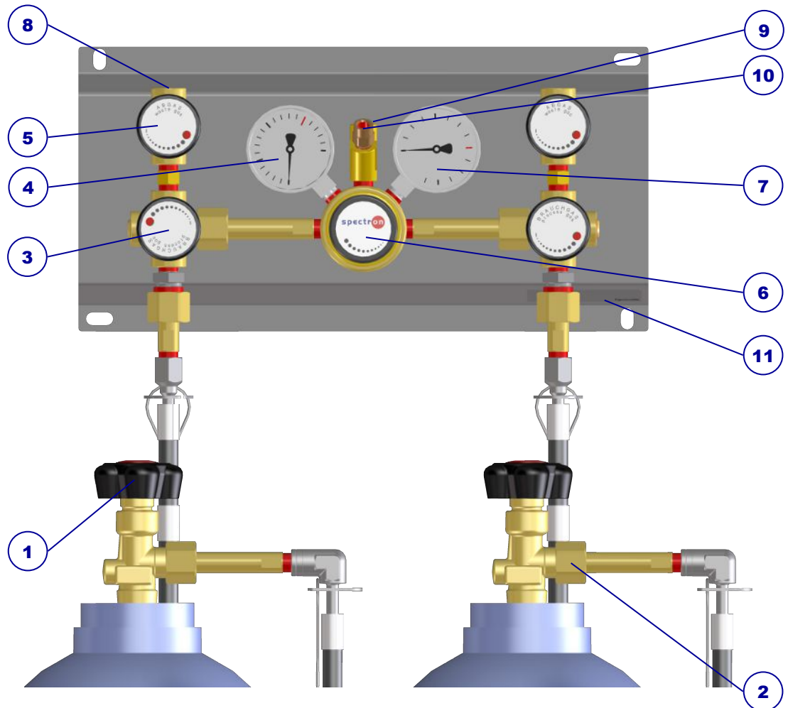
Illustration 1: Pressure control panel design CRS2000-2
