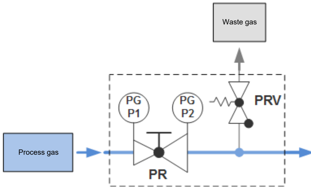
Illustration 2: P&ID U15
