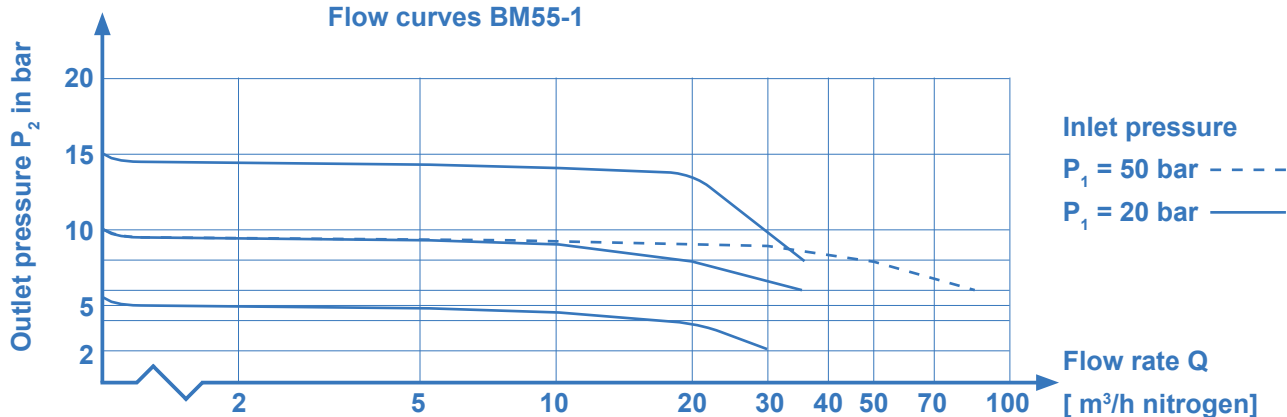
Flow curves BM55-1
