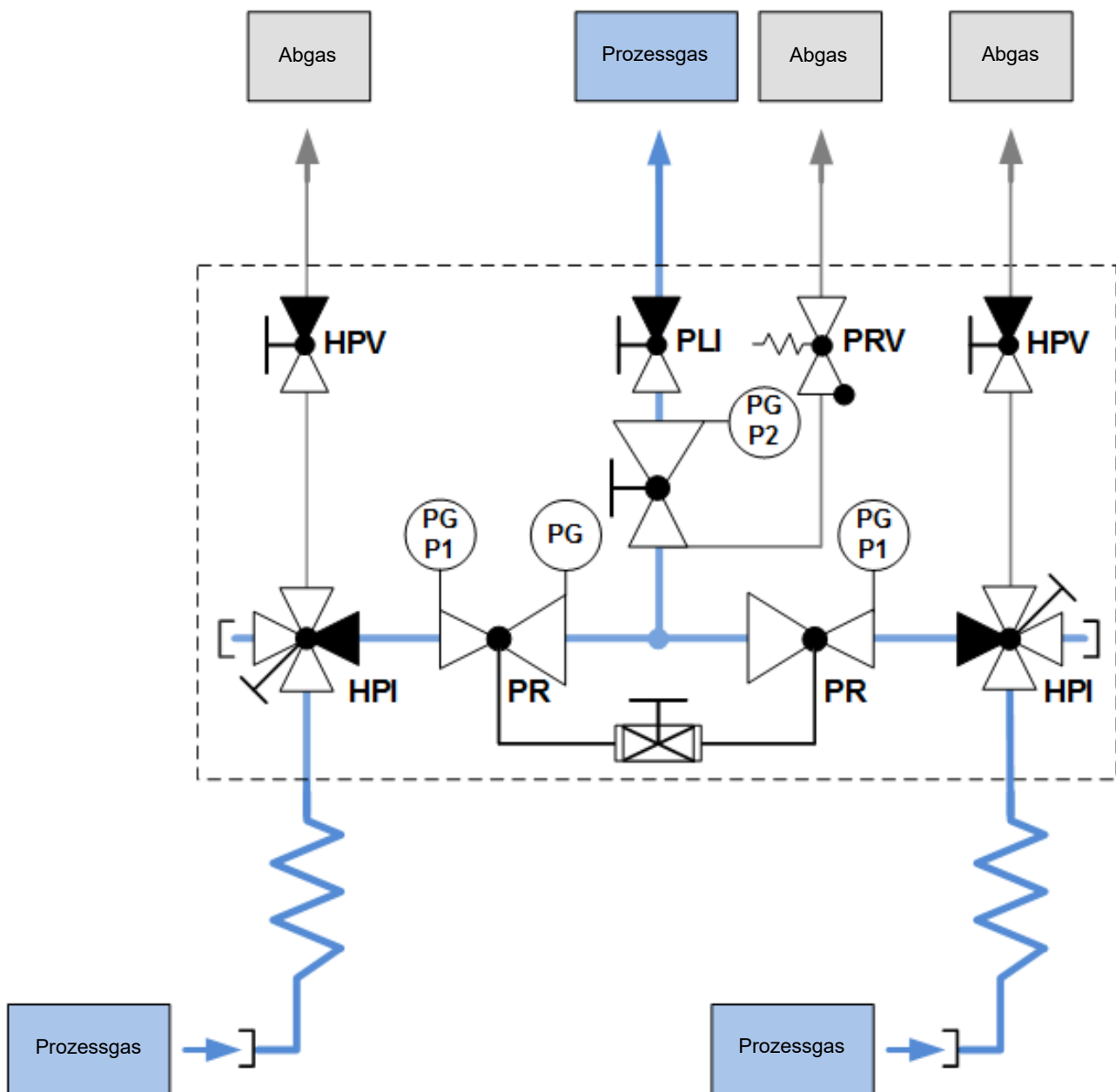
Abb. 2: Schema BM56-2U
