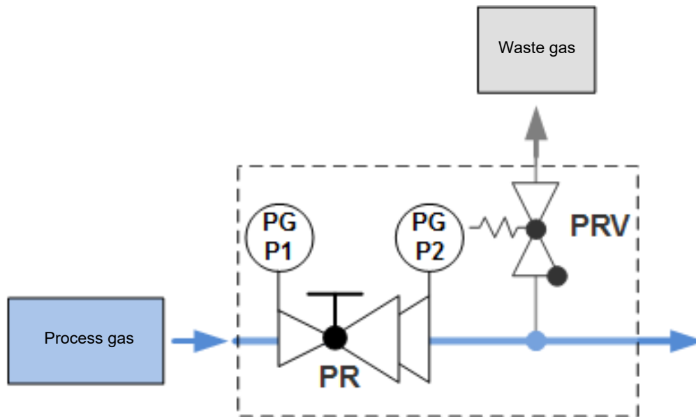
Illustration 2: P&ID M53
