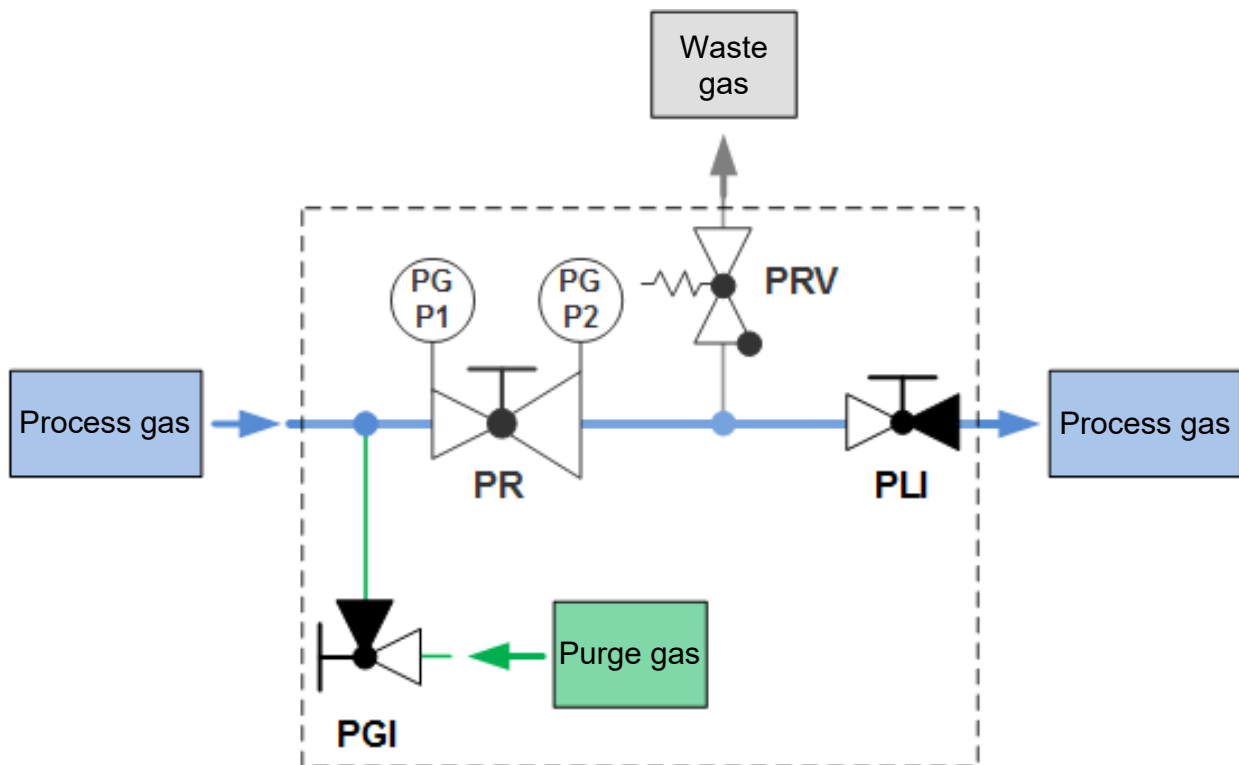
Illustration 2: P&ID FE121
