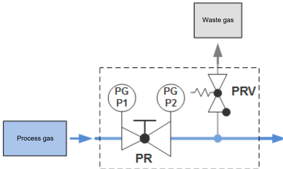
Illustration 2: P&ID E52
