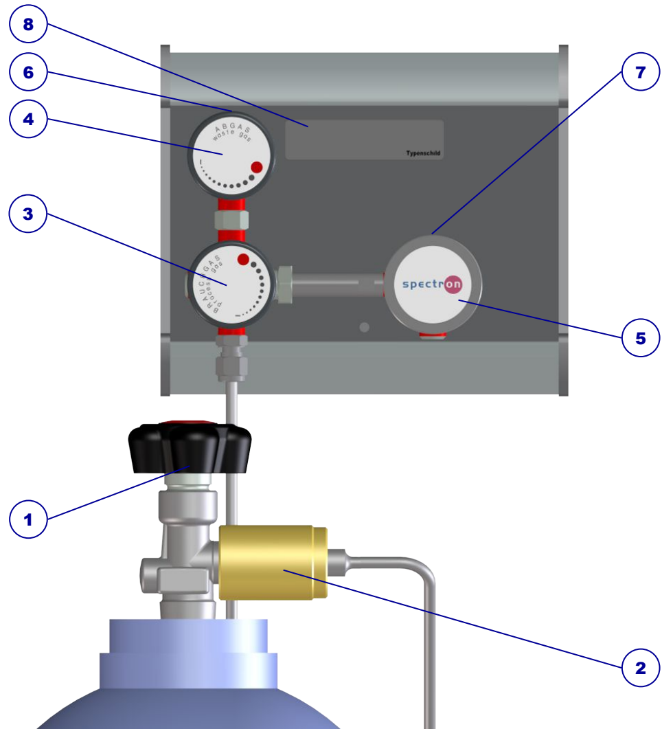
Illustration 1: BM/BE50-1 design
