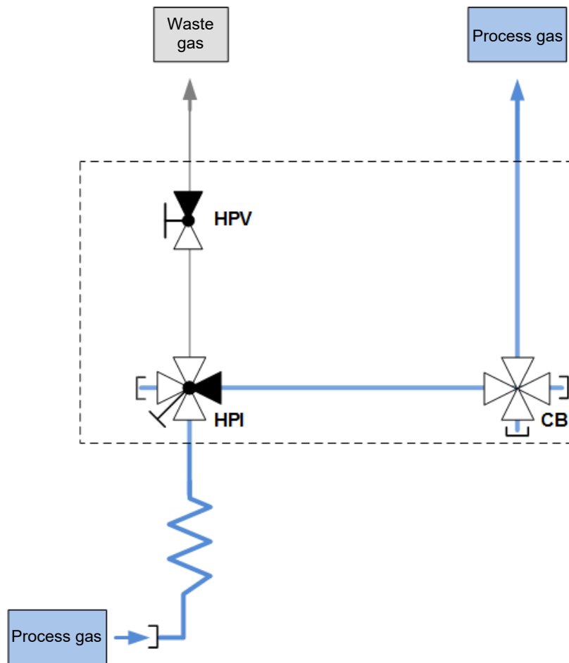
Illustration 2: P&ID BM/BE50-1
